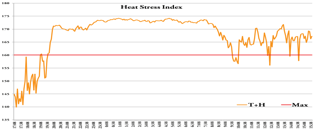
Figure 5: Example of the Heat Stress Index (°F). When the sum of RH plus temperature (°F) exceeds 160 (107 for °C) birds are likely to experience heat and humidity discomfort.
